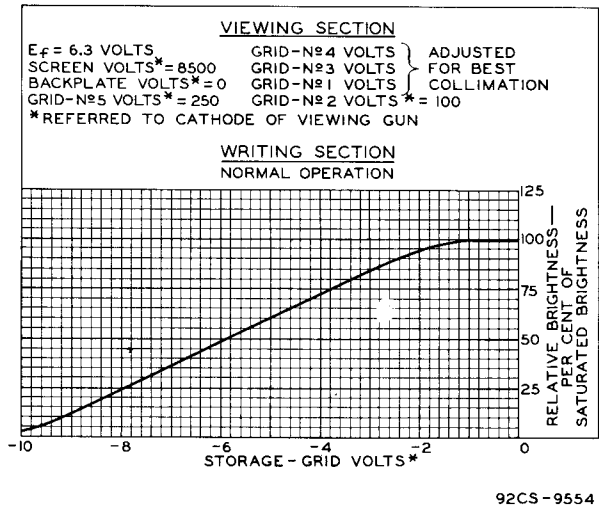
Fig.4 - Typical Storage-Grid Characteristic of Type 7183.
