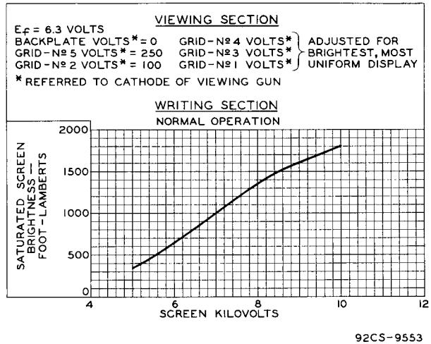
Fig.3 - Typical Characteristic of Type 7183.
